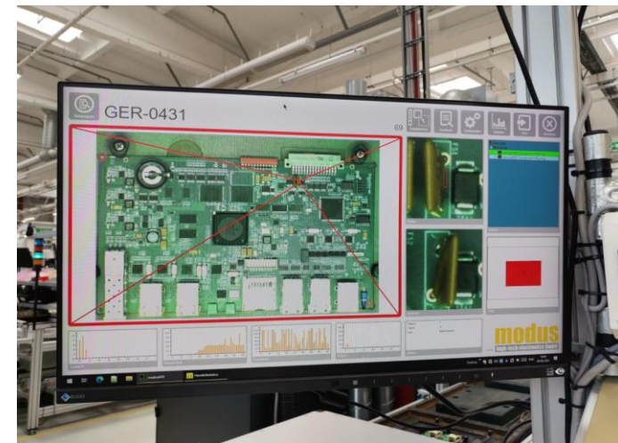
Modus AOI THT pre-wave system
